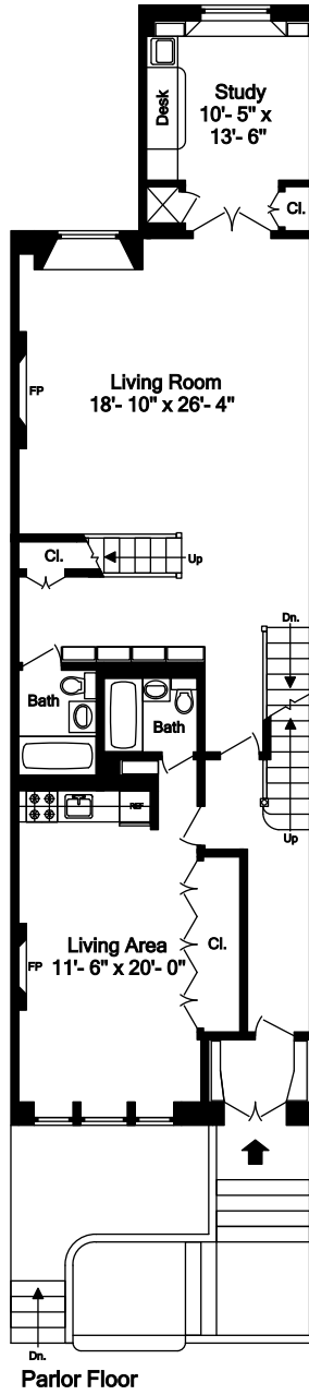
Parlor Floor
